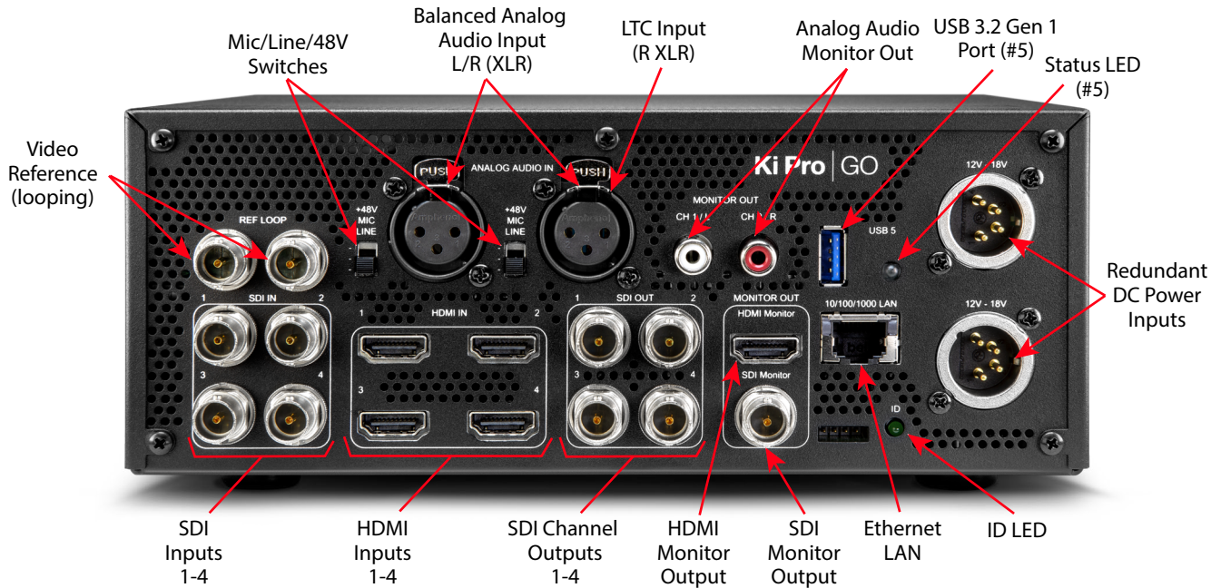
Figure 5. Ki Pro GO Rear Panel
