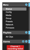
Figure 22. Alarms Pane
