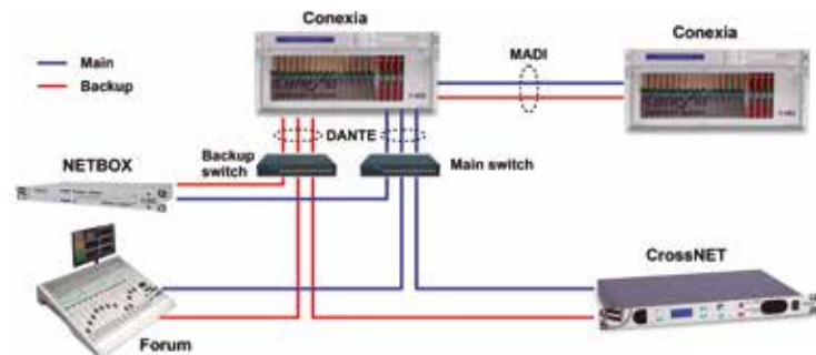
Redundant diagram with multi-channel cards to console and matrix
