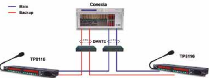
Diagram connection to panels, redundant via Dante™ network
